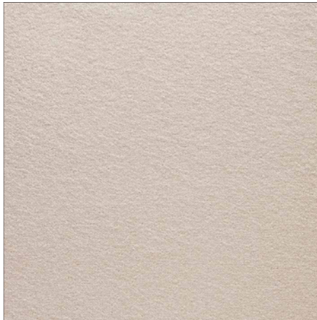
102 Milky Way
